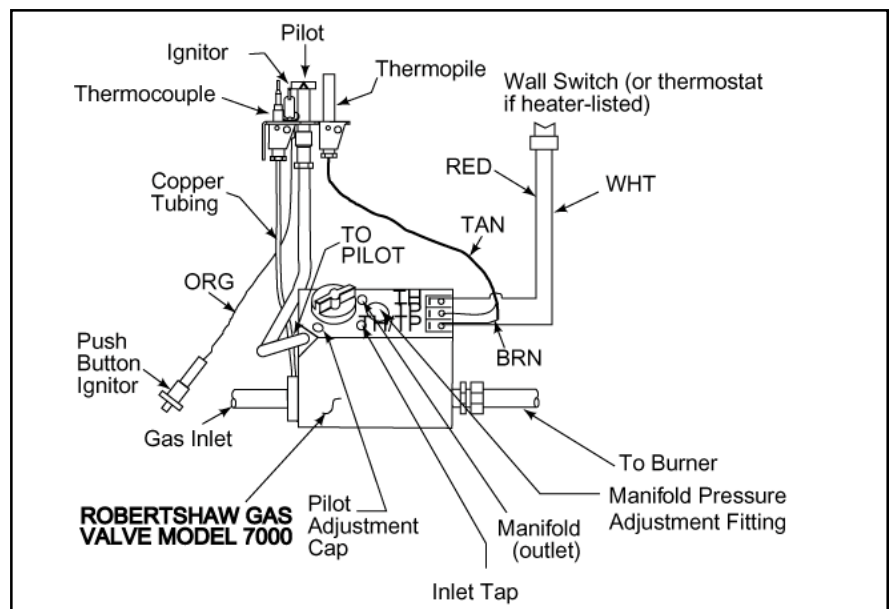
Figure 39 - Standing Pilot Ignition Wiring Diagram
