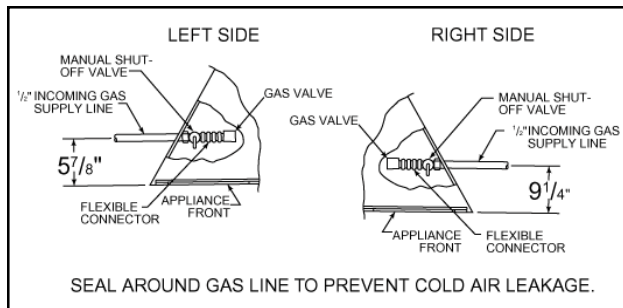
Figure 38 - Gas Line
