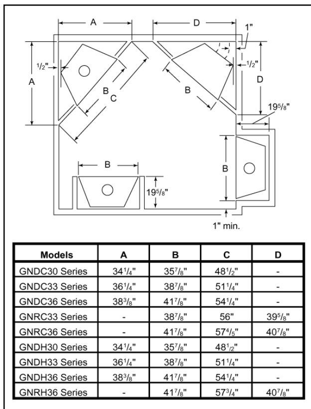
Figure 3 Appliance Locations
