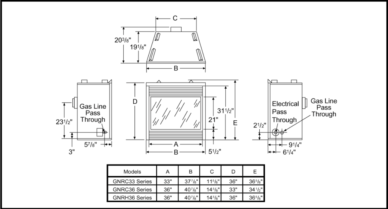
Figure 1 - Rear Vent Appliance Dimensions
