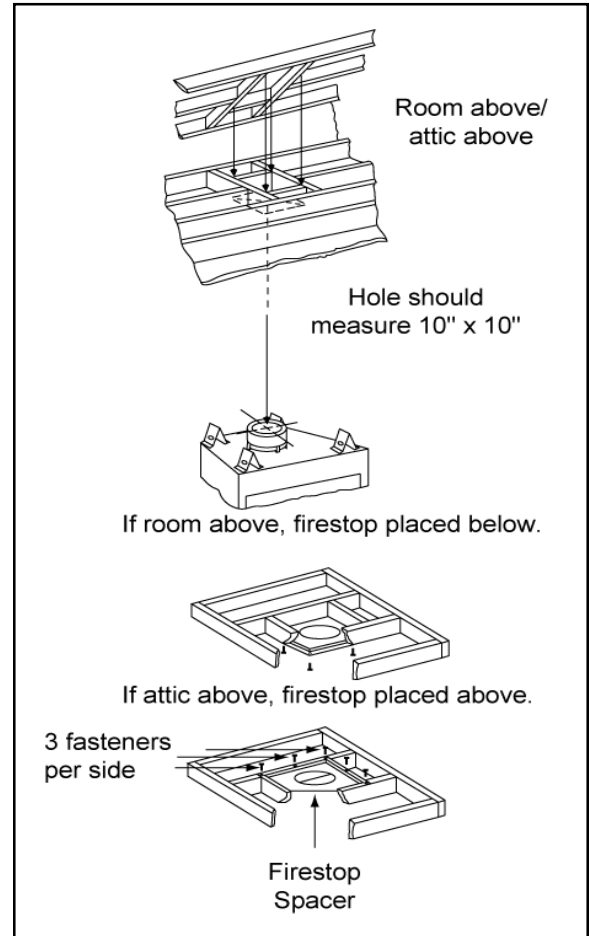
Figure 29 - Installing the Firestop Spacer
