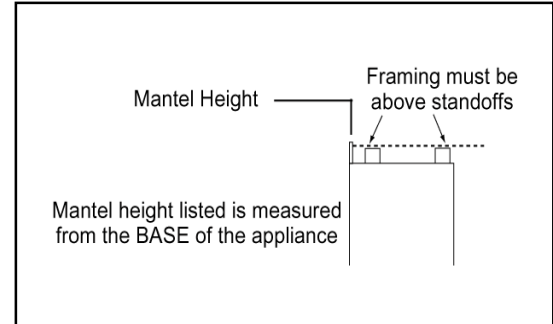
Figure 6 - Mantel Heights
