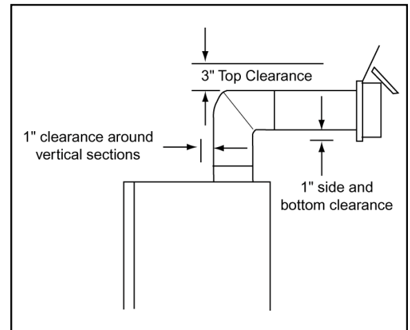
Figure 12 - Clearances
