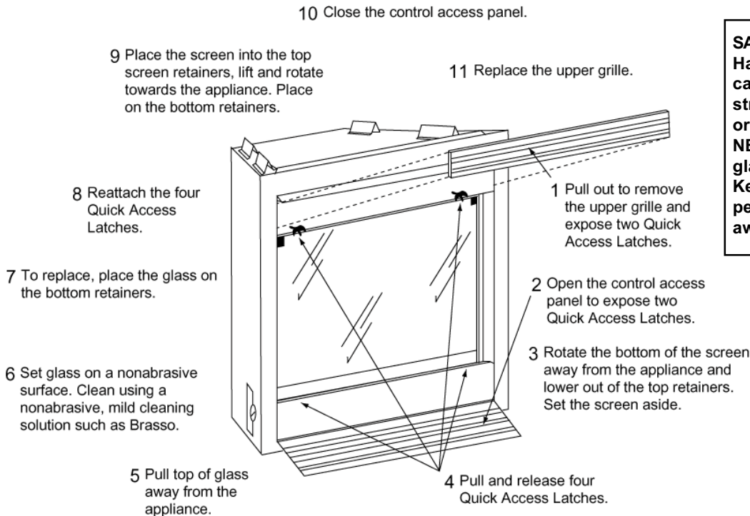
Figure 55 - Glass Cleaning
