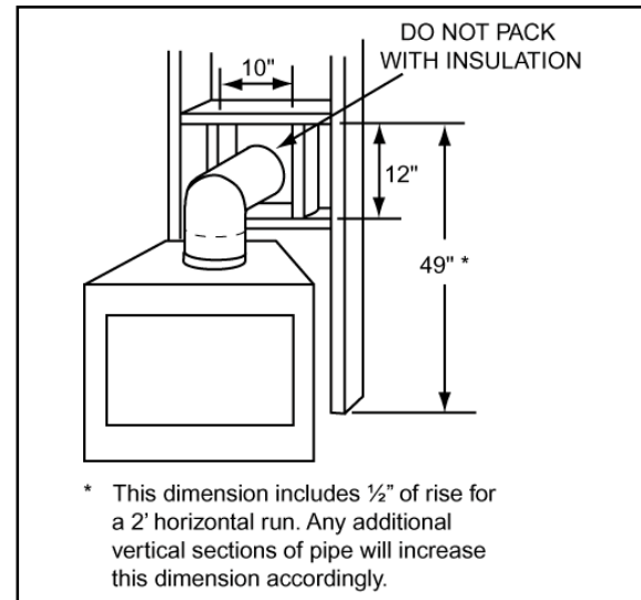
Figure 25 - Exterior Wall Hole - Top Vent
